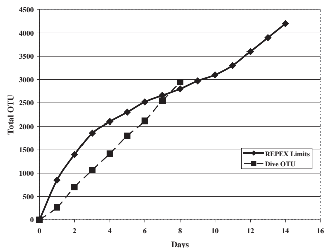
Figure 2 Allowable cumulative oxygen dose: REPEX limits and cumulative oxygen dose (OTU) for expedition divers (see text for explanation)
